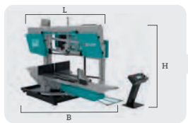
KS 1202 NC B 1950 mm L 4000 mm H 2750 mm h 855 mm Kg 3550
