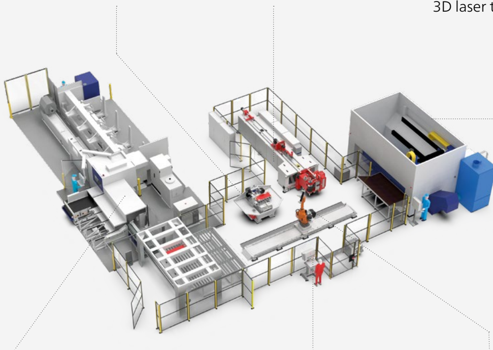
TRUMPF TruLaser Tube Laser tube cutting machine
